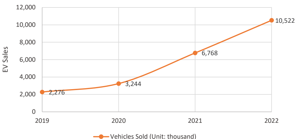
Fig 1. Global EVs Sales 2019 - 2022
