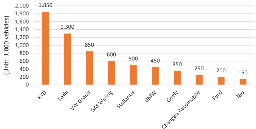
Fig 3. Global EV Sales By OEM in 2022
