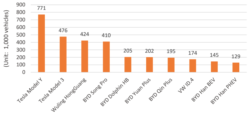
Fig 4. EV Models Global Sales in 2022
