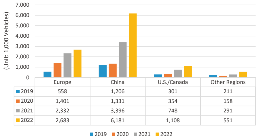
Fig 2. EV Sales 2019- 2022 by Regions
